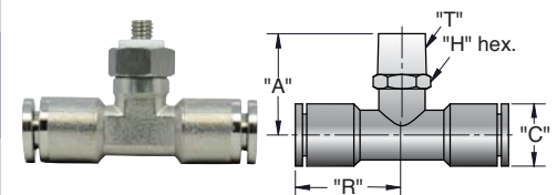
Branch Tee
