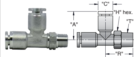
Run Tee
